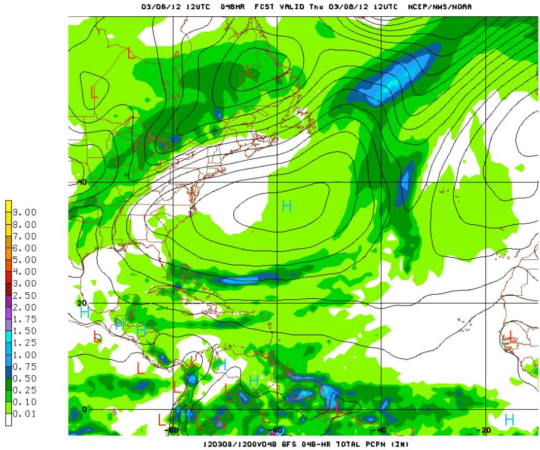
Fig. 3 GFS 24 hour rainfall accumulation ending 6:00 am Thu. Mar. 8, 2012, forecasting amounts of 0.25-0.50 of-an-inch over central and northern coast
