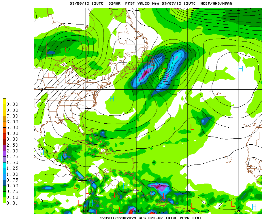
Fig. 1 GFS 24 hour rainfall accumulation ending 6:00 am Wed. Mar. 7, 2012, forecasting amounts of 0.75-1.00 inch, especially over central and northern coast.
